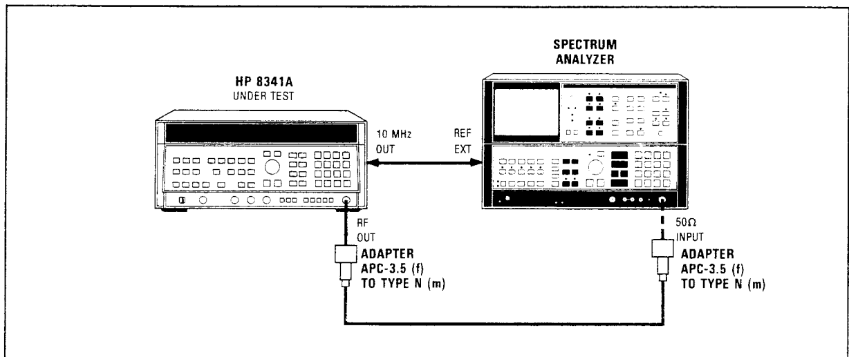
Figure 4-7. Spurious Signals Test Setup (10 MHz to 20 GHz)
