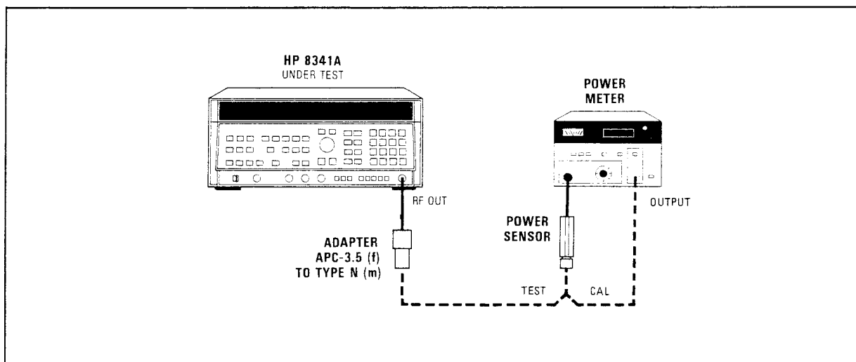
Figure 4-10. Power Sweep Test Setup
