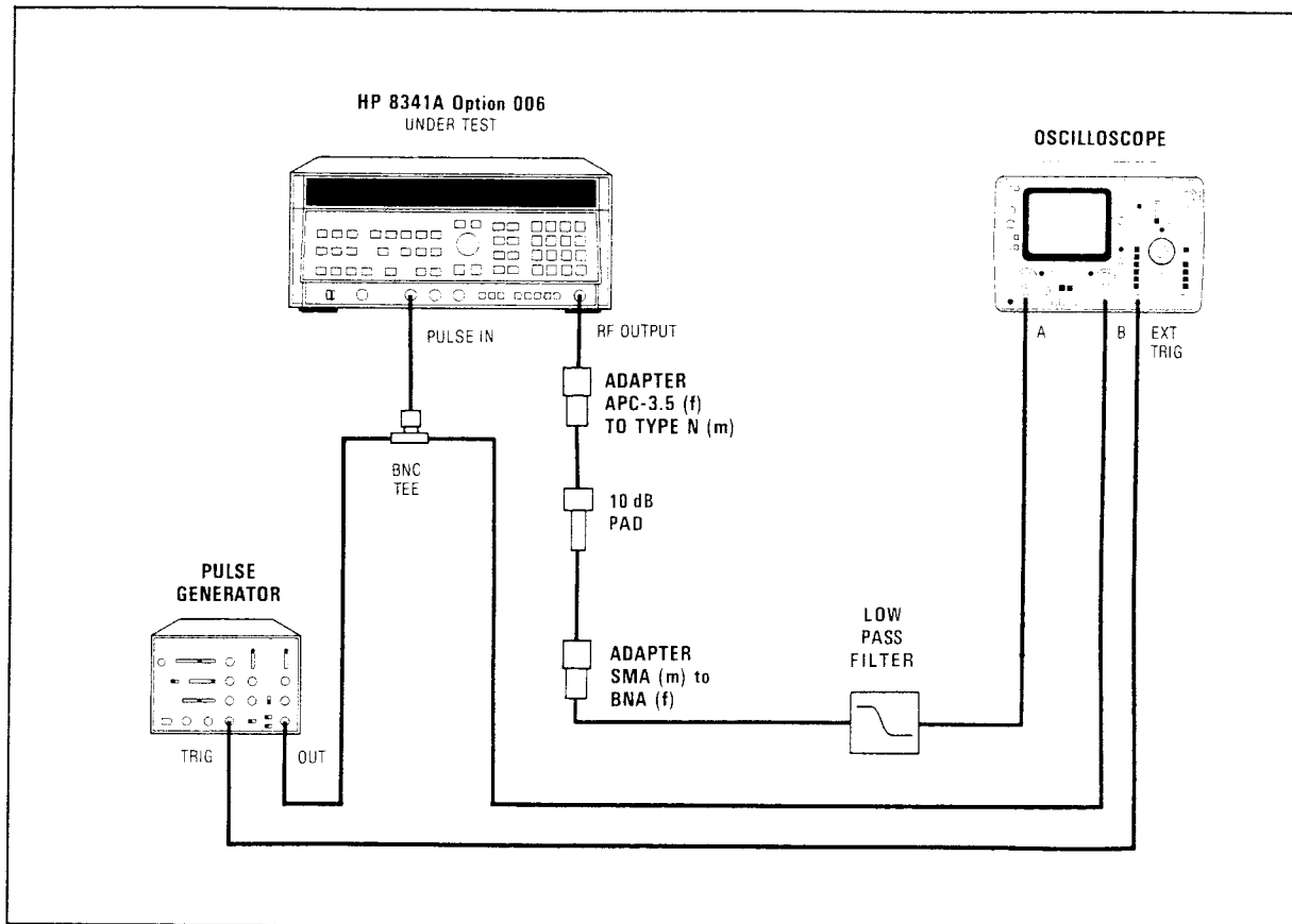
Figure 4-17. Pulse Modulation Video Feedthrough Test Setup
